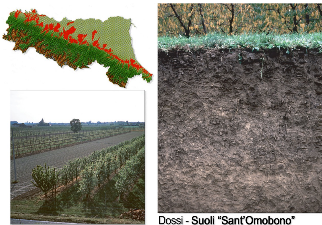
Figure 8. Reliefs of the alluvial plain: area, landscape and profile of a representative soil.
