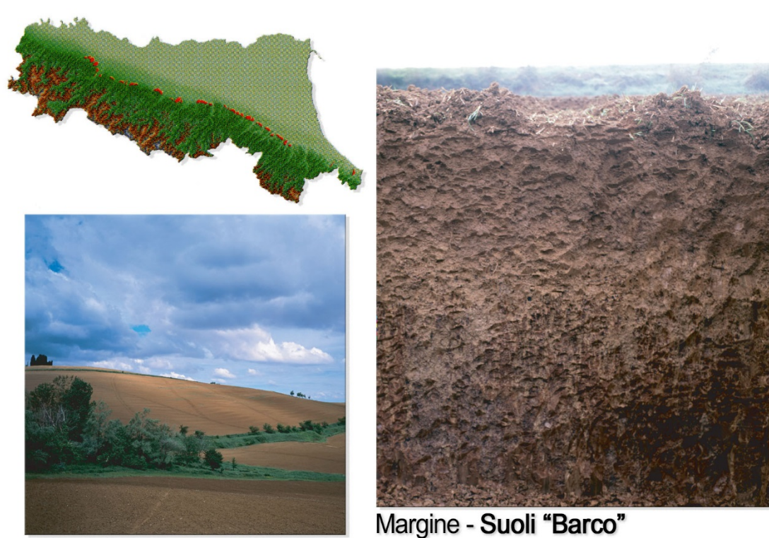
Figure 9. Apennine margin: area, landscape and profile of a representative soil.
